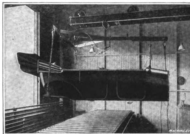
Fig. 10—In some cities municipal regulations prohibit extending a beam out over the roadway to support a trolley. The Palmer-Bee Co., of Detroit, Mich., made a movable trolley for the Palge-Detroit Motor Car Co., which can be run out over the road to pick up auto bodies
